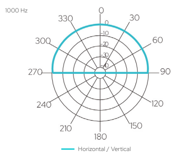
Horizontal/vertical polar diagrams
